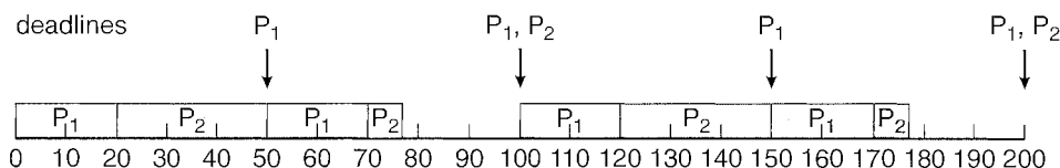
Figure 19.8 Rate-monotonic scheduling.
